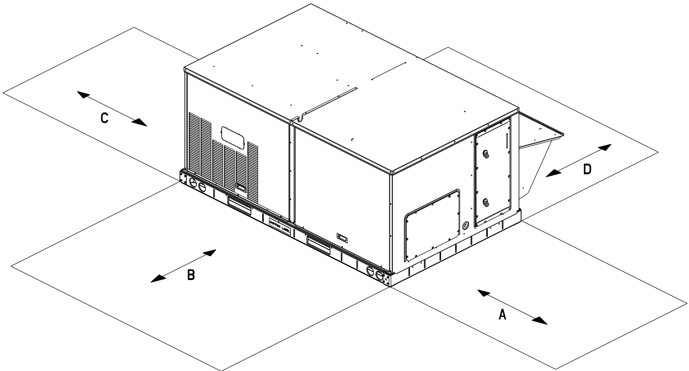
Fig. 6 - Service Clearance Dimensional Drawing
